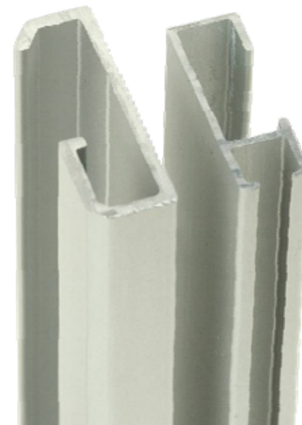
Open-faced (left) and Close-faced tracks Note: The mounting surface would be to the right.
