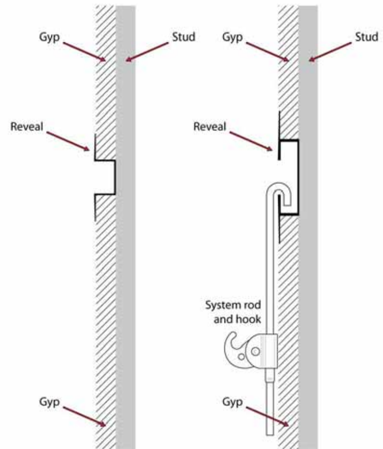
Common reveal without flanges and a compatible reveal with a P-End hanging system rod placed on the flange ready to suspend a wall object.
